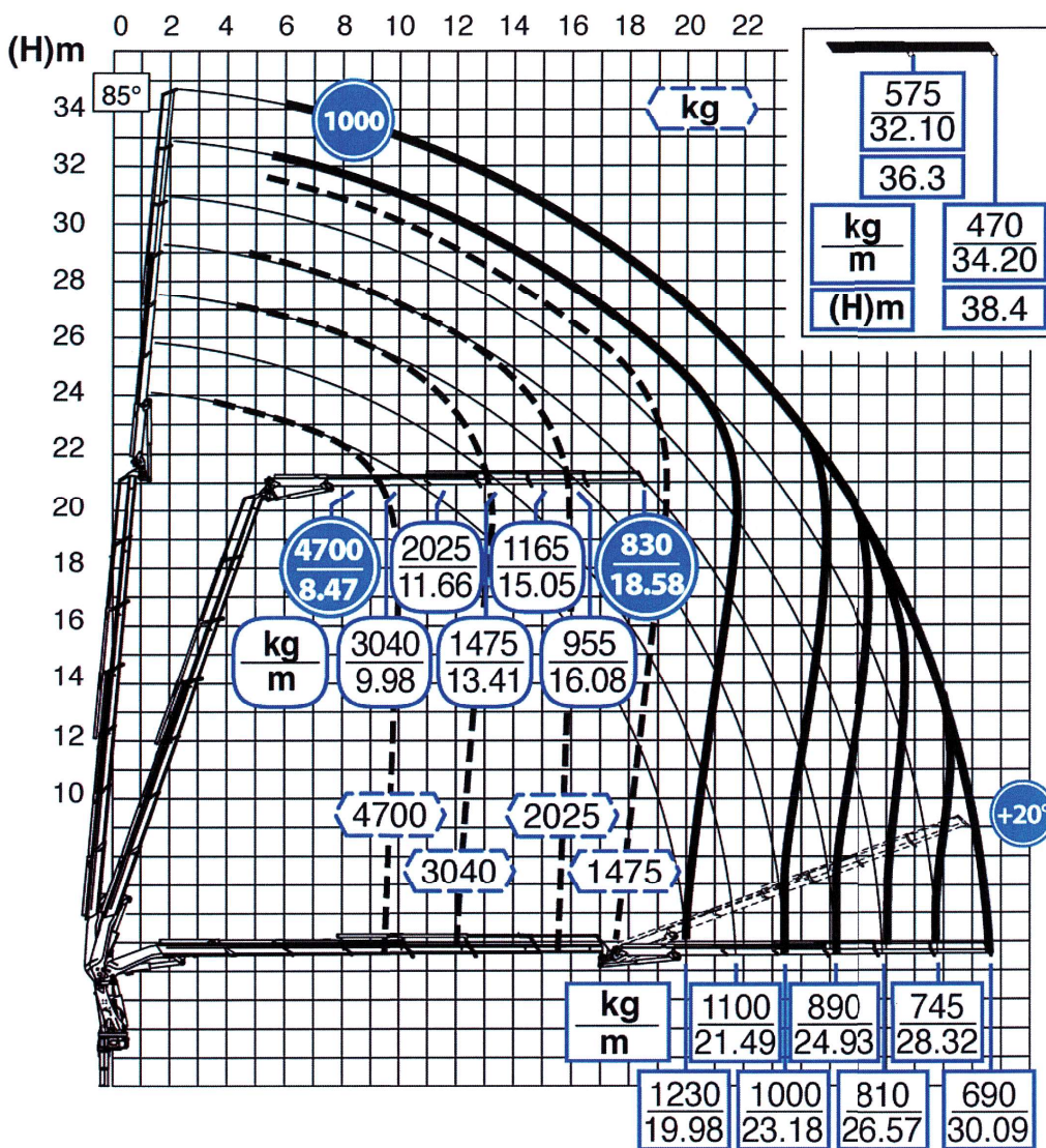
EFFER 655 - DIAGRAMM 6S JIB 6S HEAVY DUTY
